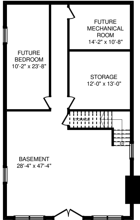
BASEMENT PLAN
