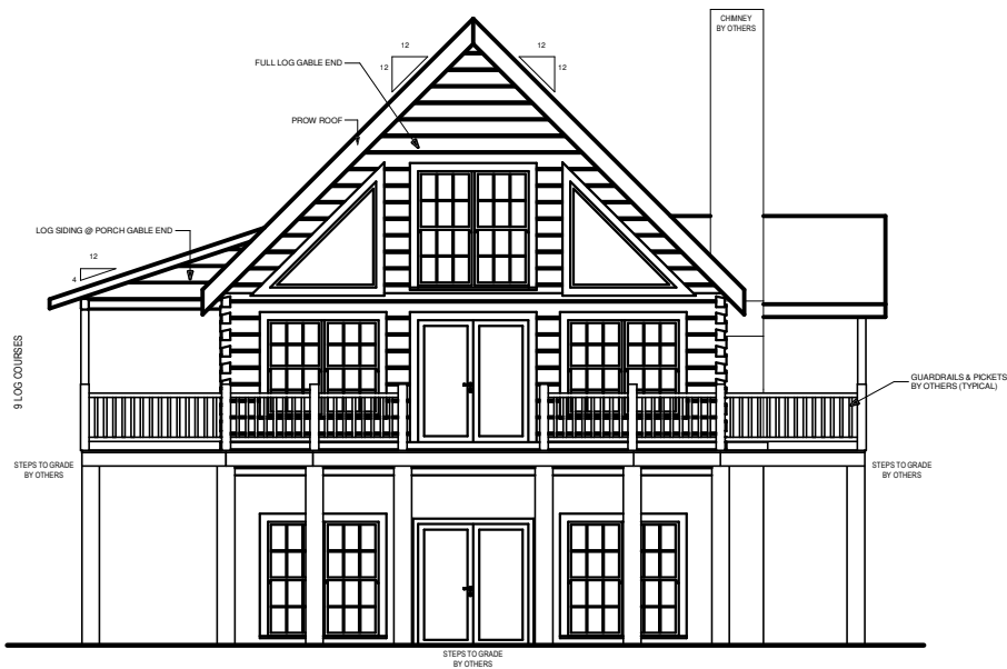
FRONT ELEVATION
