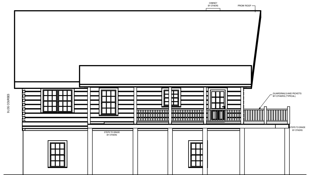
LEFT ELEVATION
