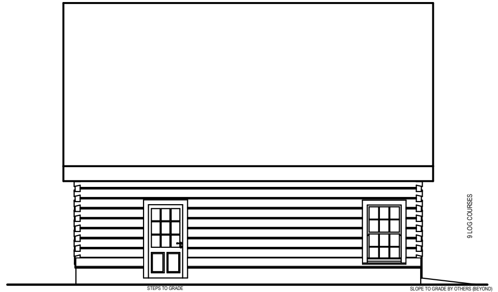
LEFT ELEVATION
