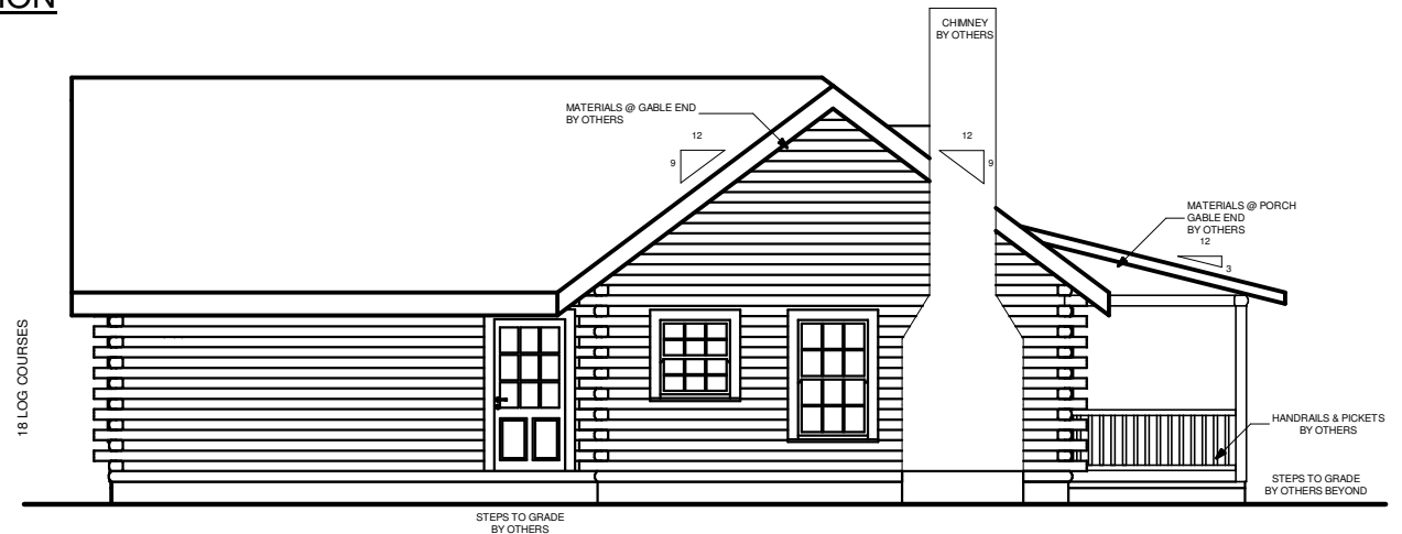
LEFT ELEVATION
