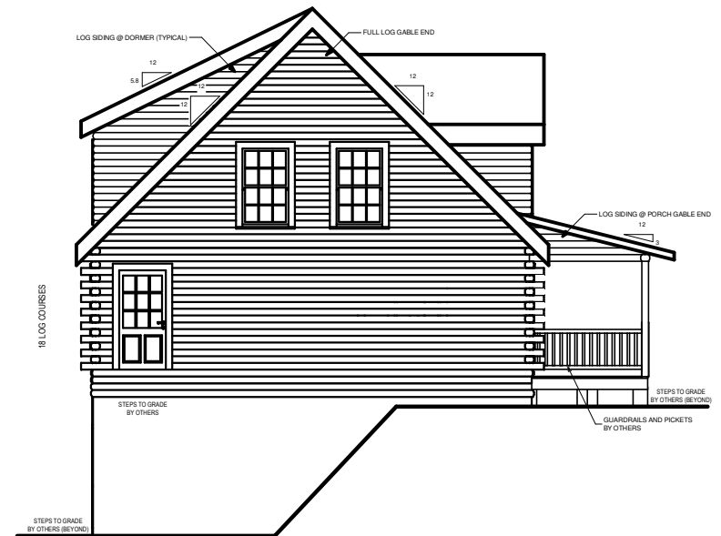
LEFT ELEVATION
