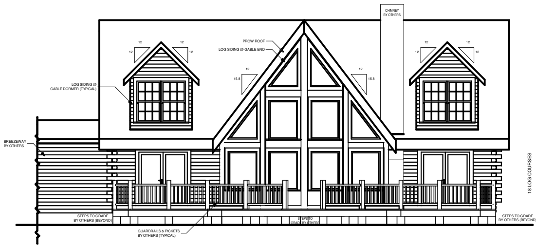
REAR ELEVATION
