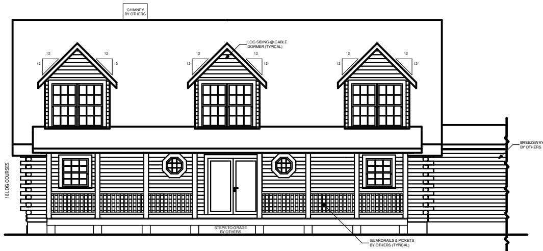
FRONT ELEVATION
