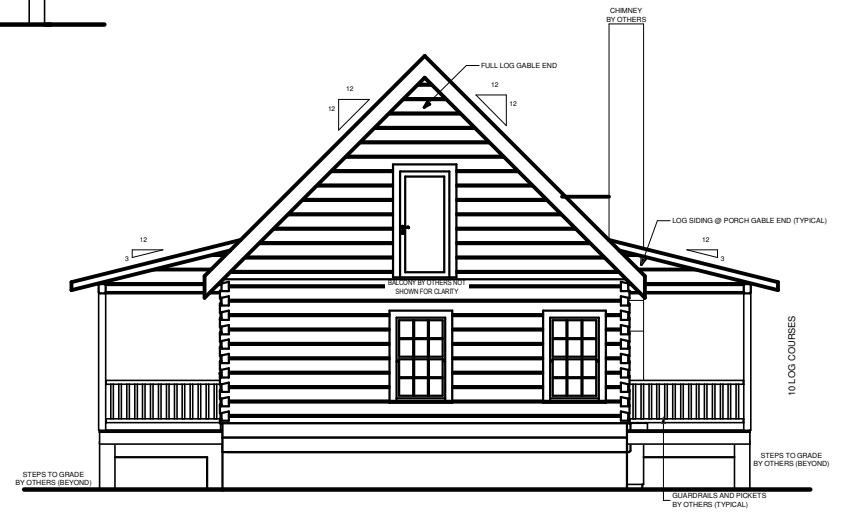
LEFT ELEVATION
