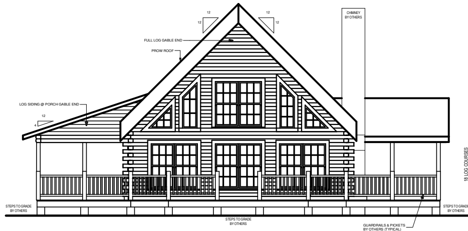
FRONT ELEVATION
