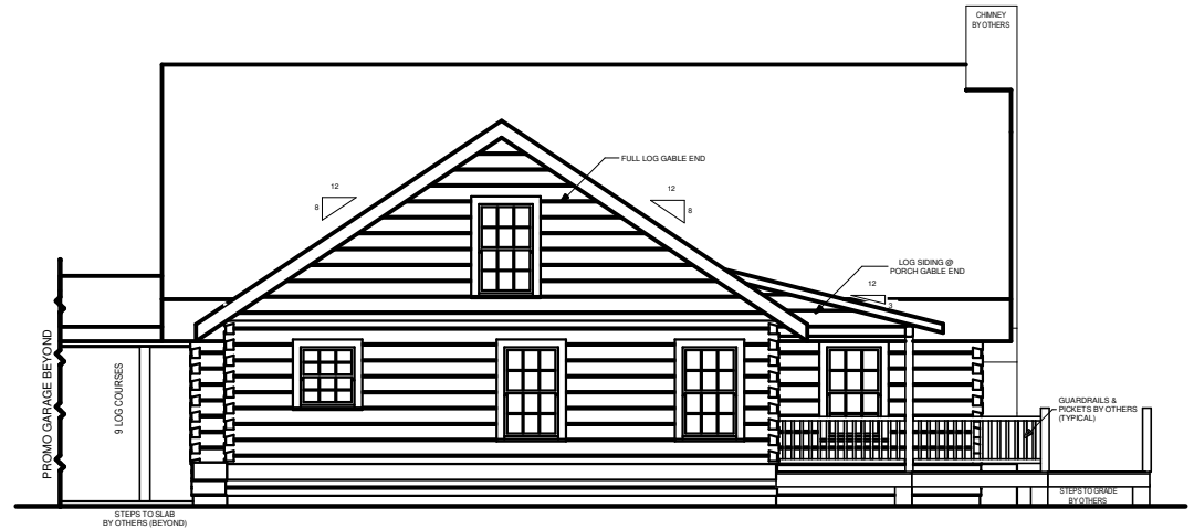
LEFT ELEVATION
