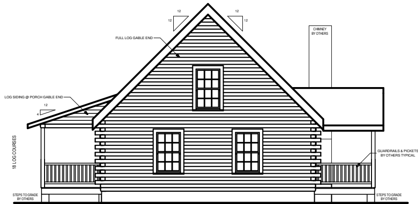
REAR ELEVATION
