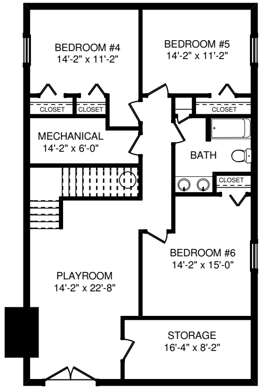
BASEMENT PLAN
