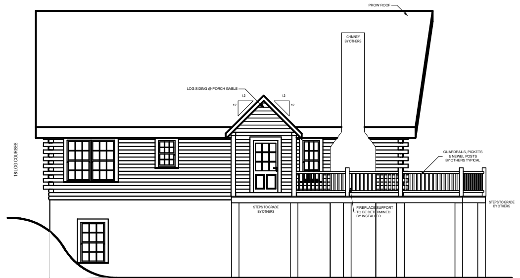
LEFT ELEVATION
