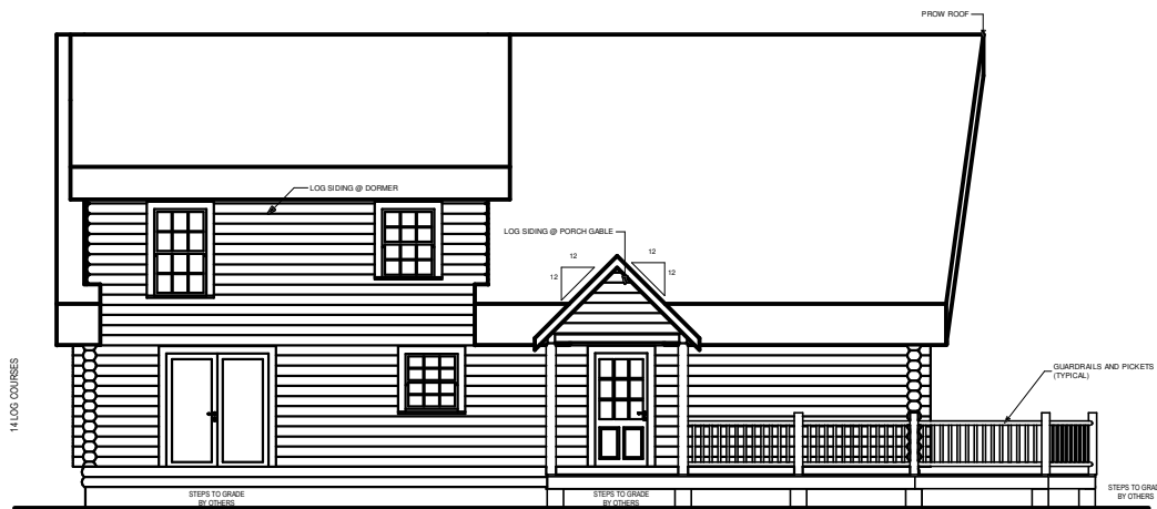
LEFT ELEVATION
