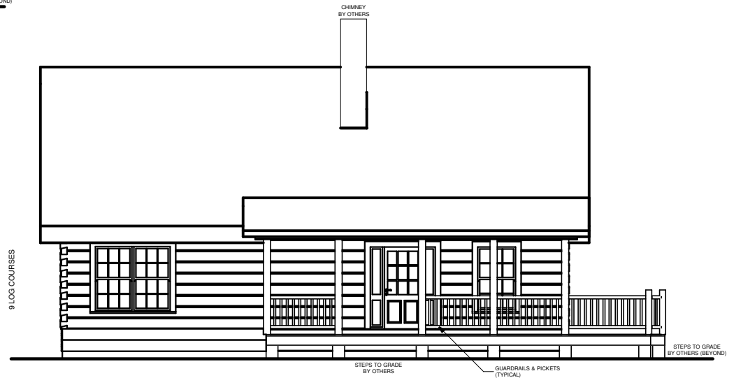
LEFT ELEVATION
