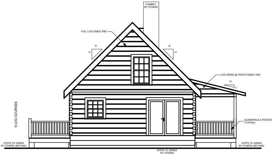
REAR ELEVATION
