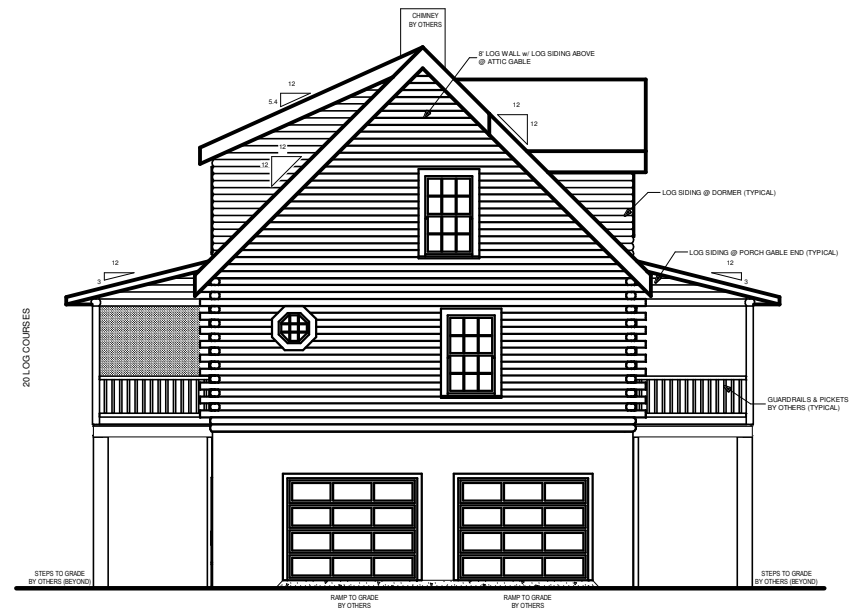
LEFT ELEVATION
