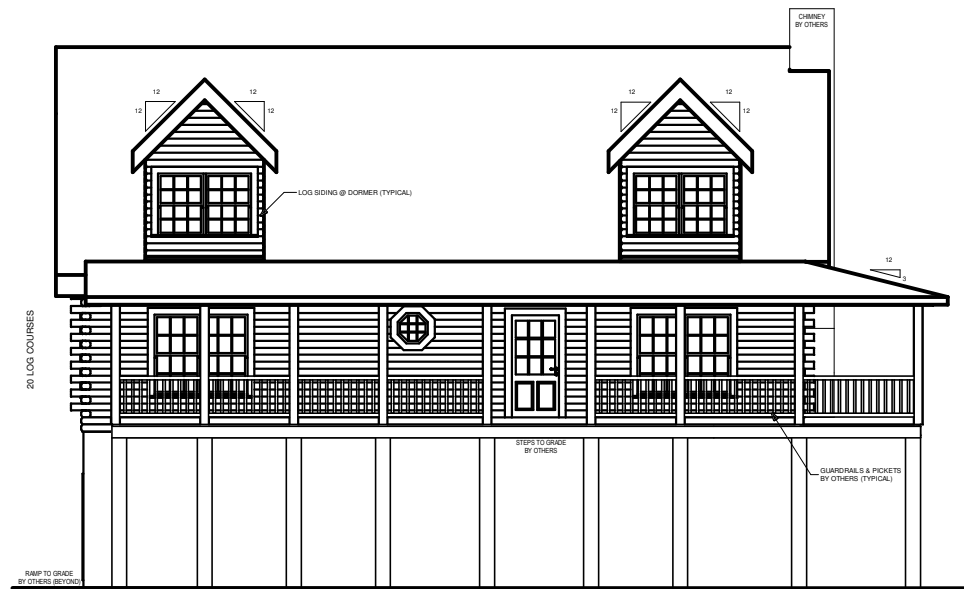
FRONT ELEVATION
