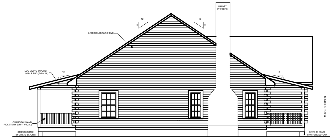
LEFT ELEVATION
