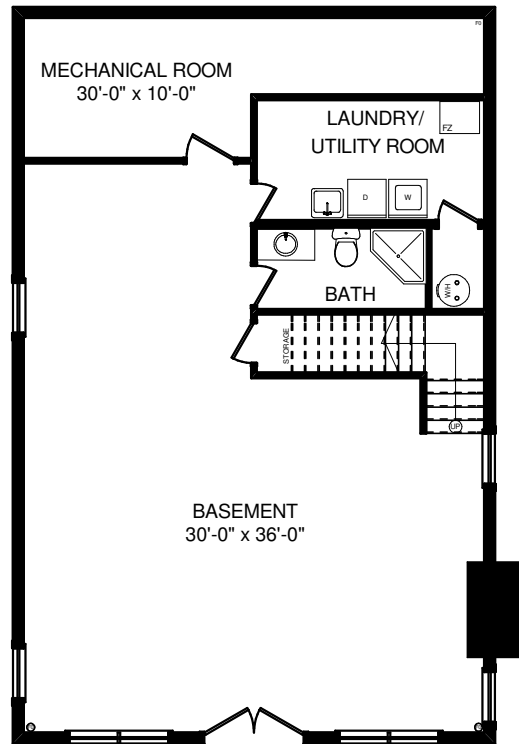
BASEMENT PLAN
