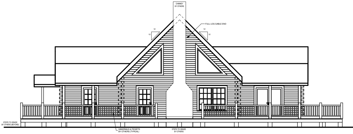
FRONT ELEVATION
