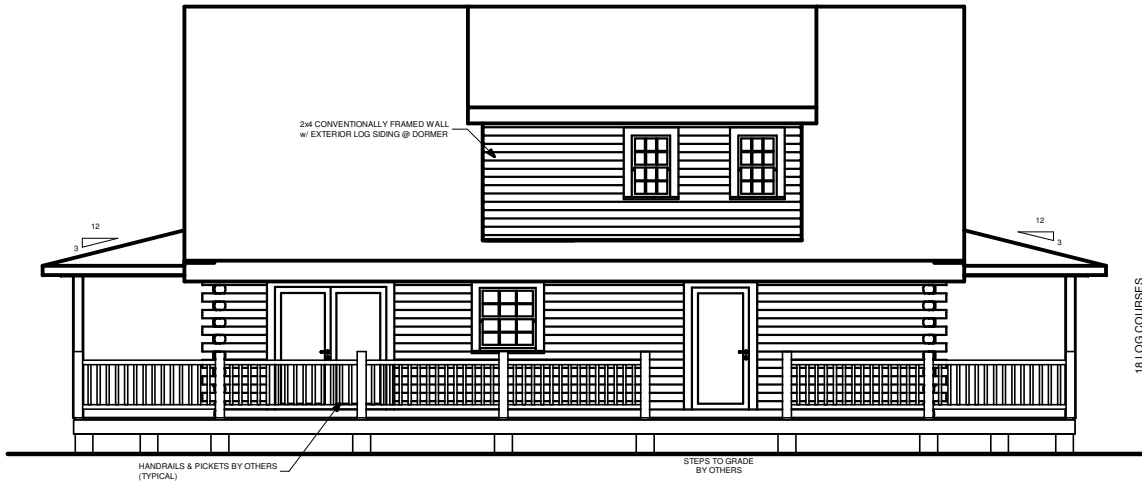
REAR ELEVATION
