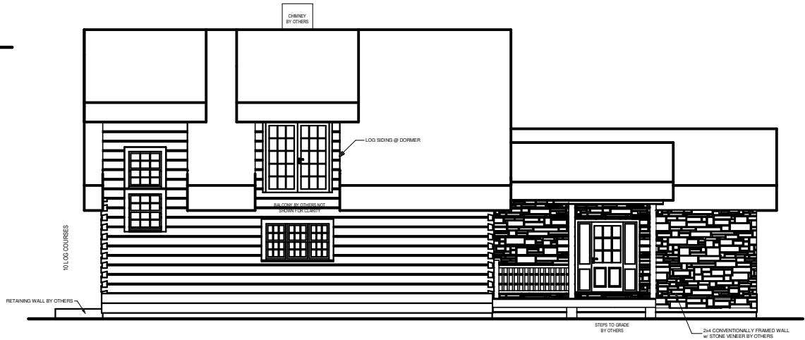
FRONT ELEVATION
