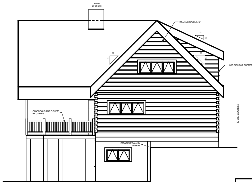
LEFT ELEVATION
