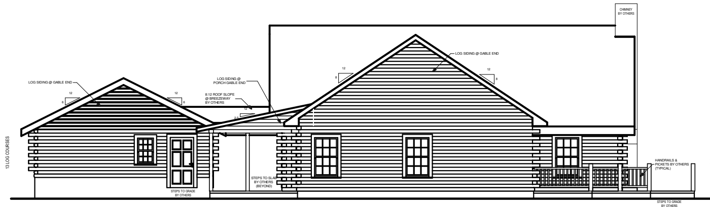
LEFT ELEVATION
