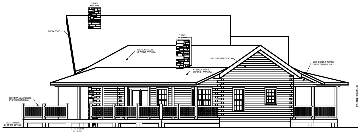
LEFT ELEVATION
