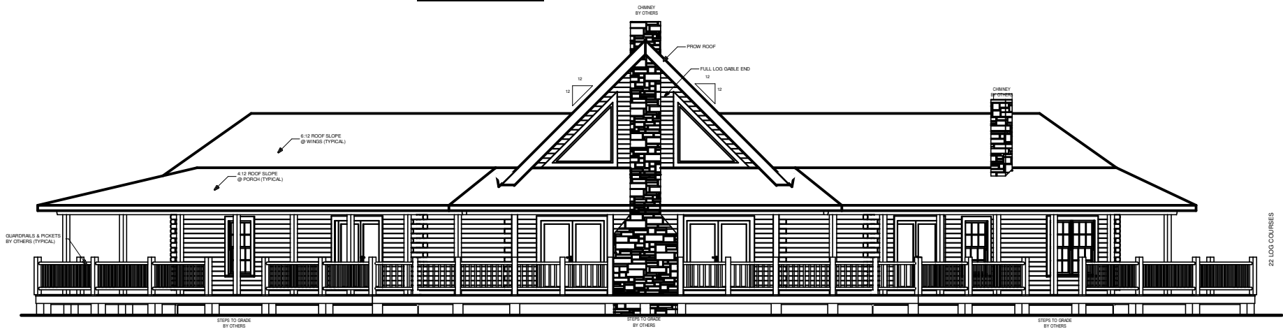
REAR ELEVATION
