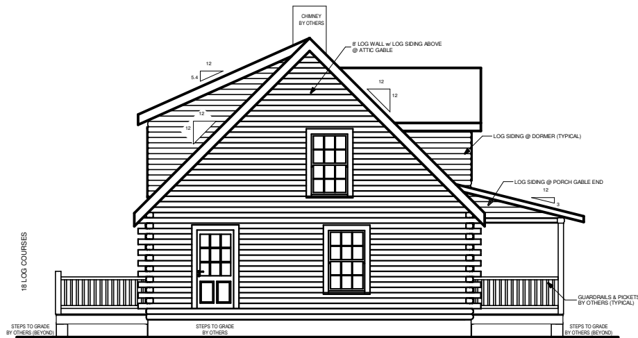
LEFT ELEVATION
