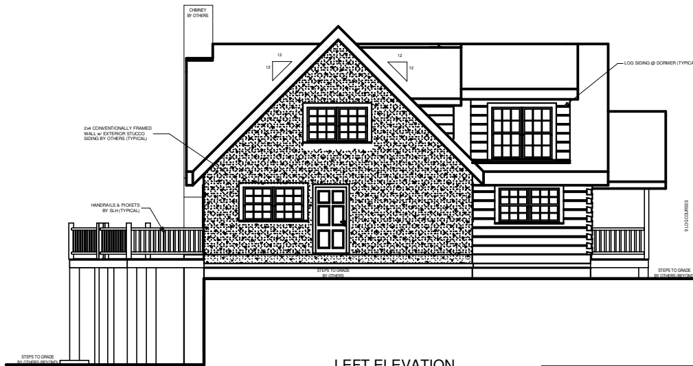
LEFT ELEVATION
