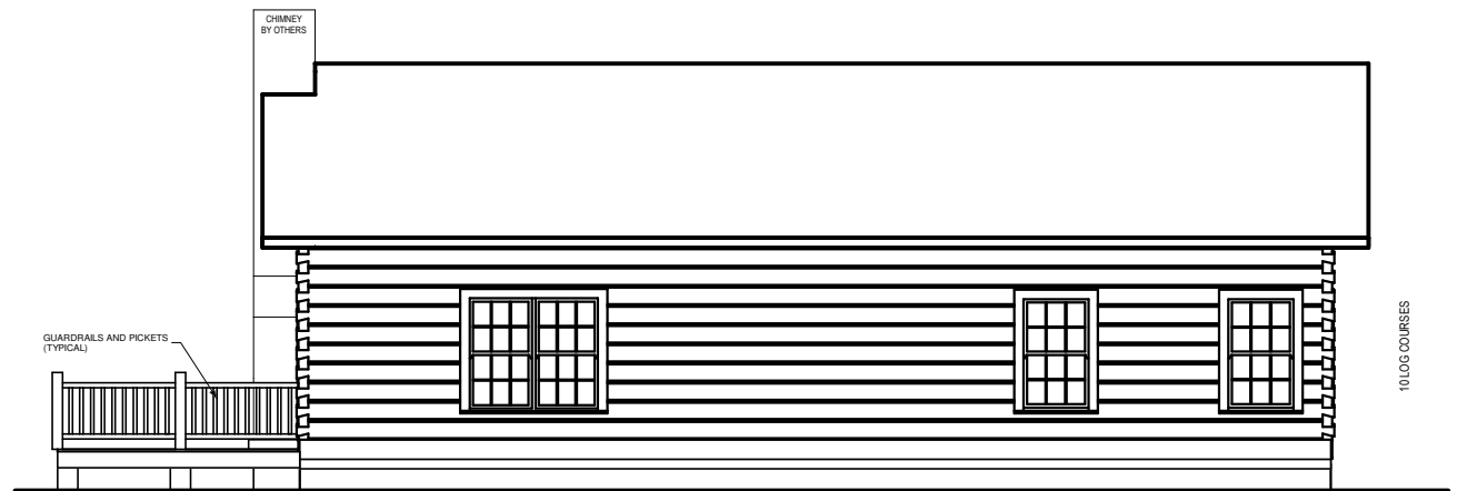
REAR ELEVATION
