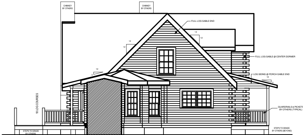
LEFT ELEVATION
