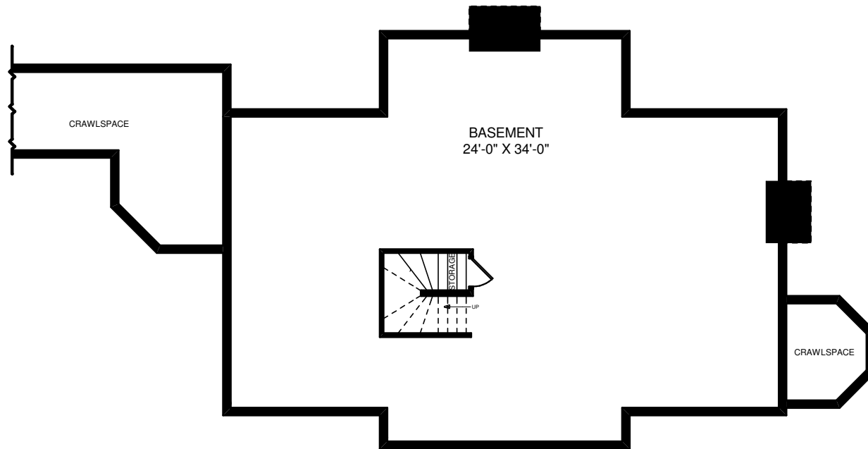
BASEMENT PLAN
