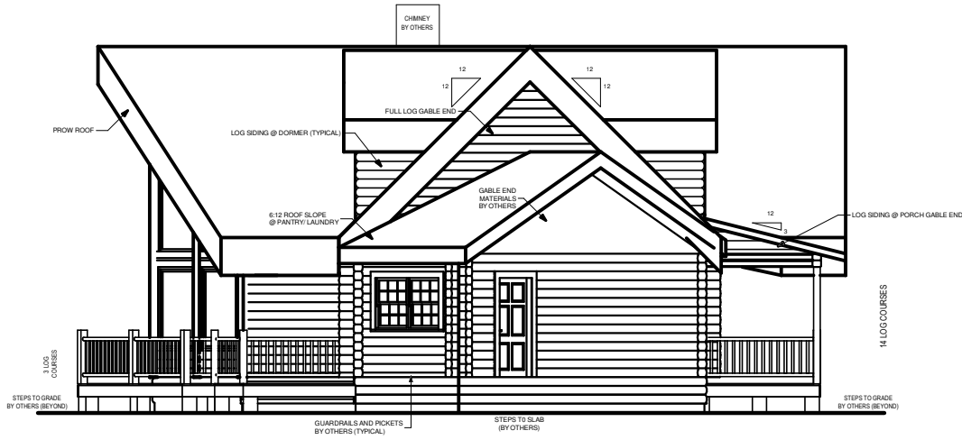
LEFT ELEVATION
