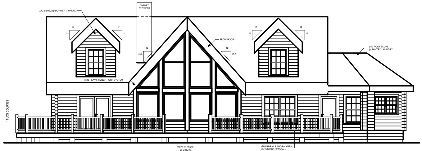
REAR ELEVATION
