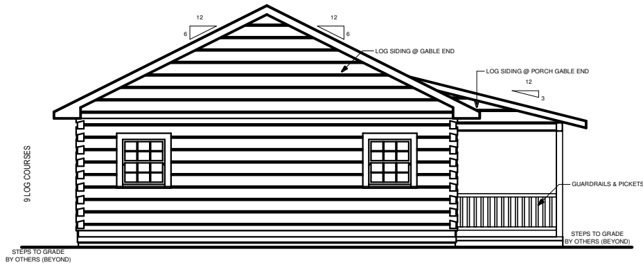
LEFT ELEVATION
