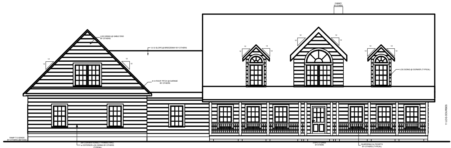
FRONT ELEVATION
