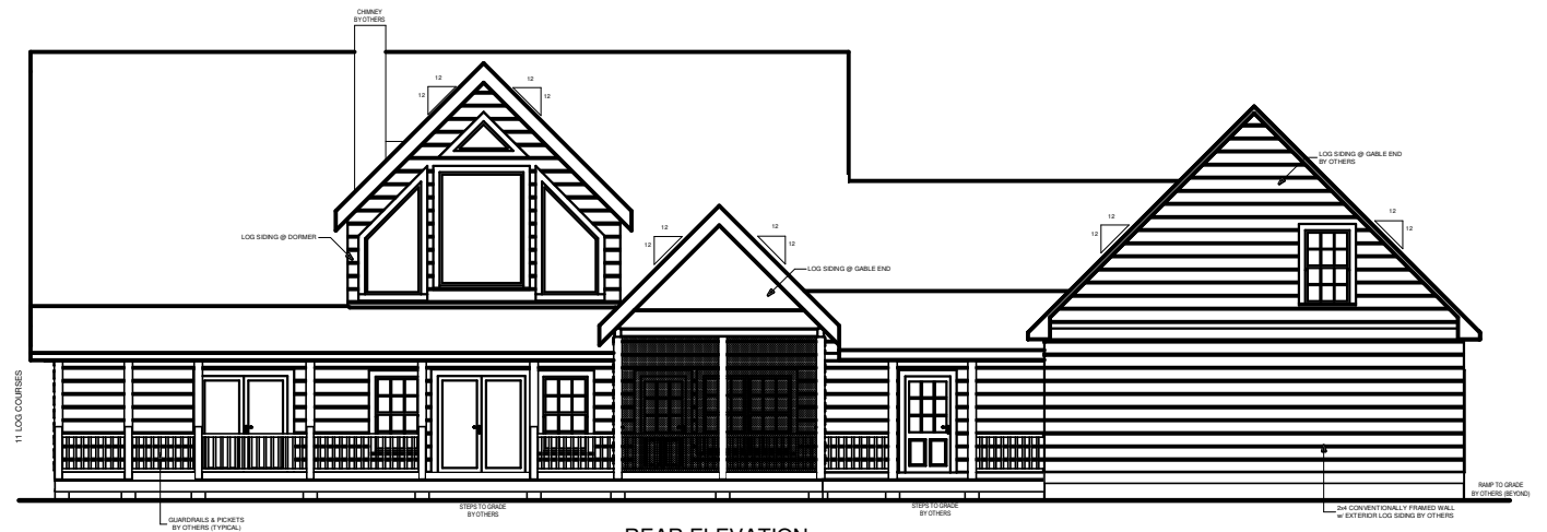
REAR ELEVATION
