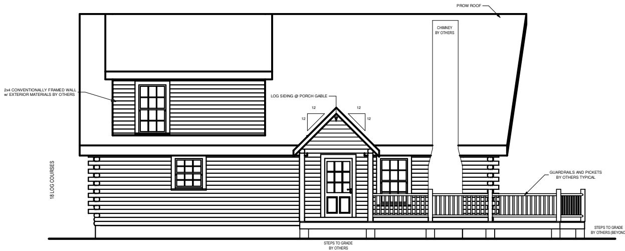
LEFT ELEVATION
