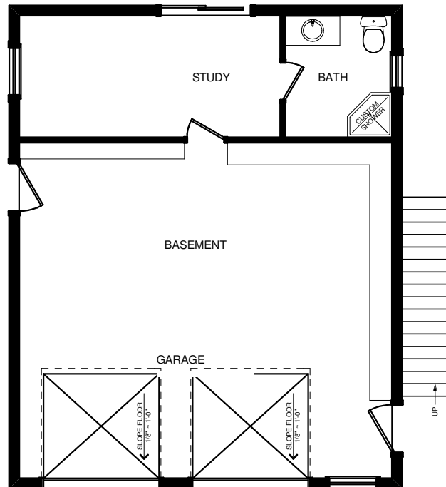
FOUNDATION PLAN
