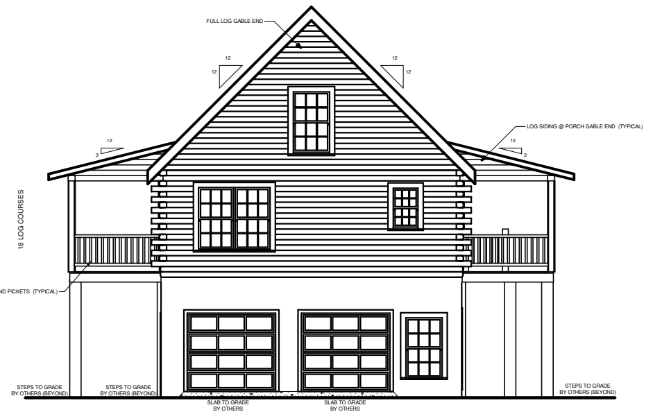
FRONT ELEVATION
