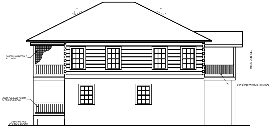
LEFT ELEVATION
