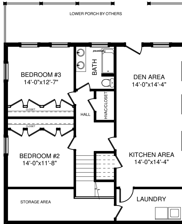
BASEMENT PLAN
