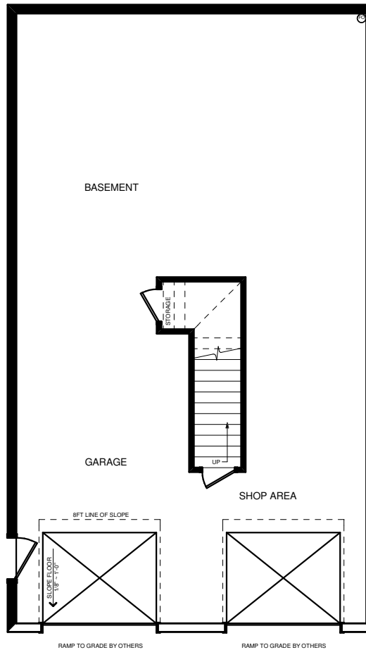
BASEMENT PLAN
