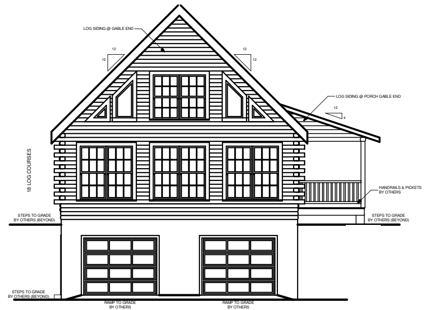
FRONT ELEVATION
