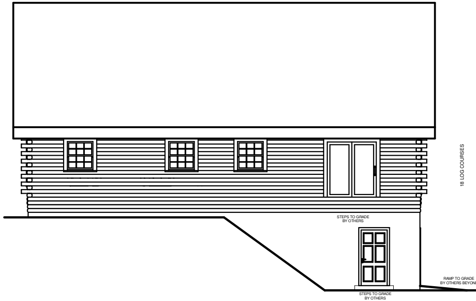
LEFT ELEVATION
