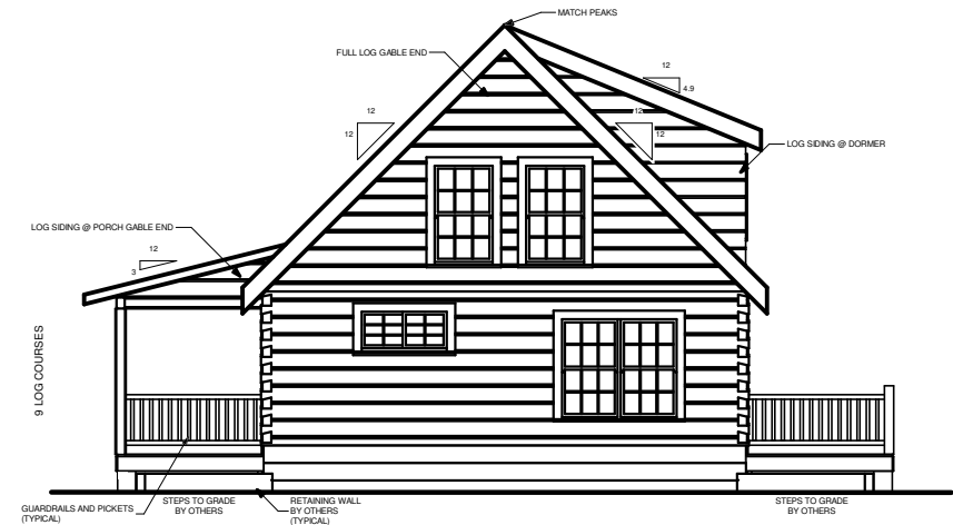
REAR ELEVATION
