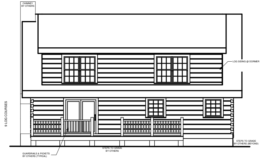
REAR ELEVATION
