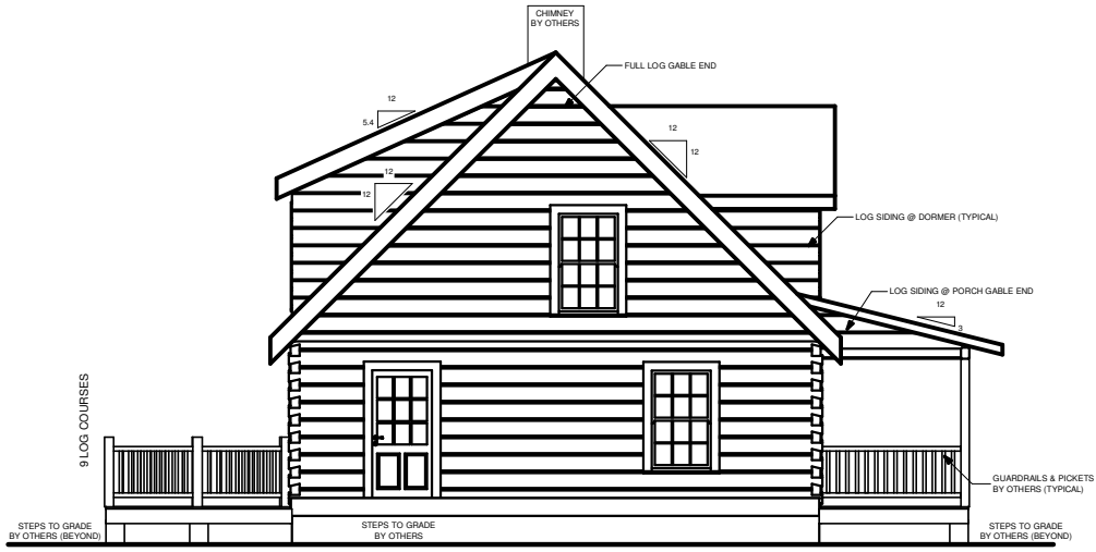
LEFT ELEVATION
