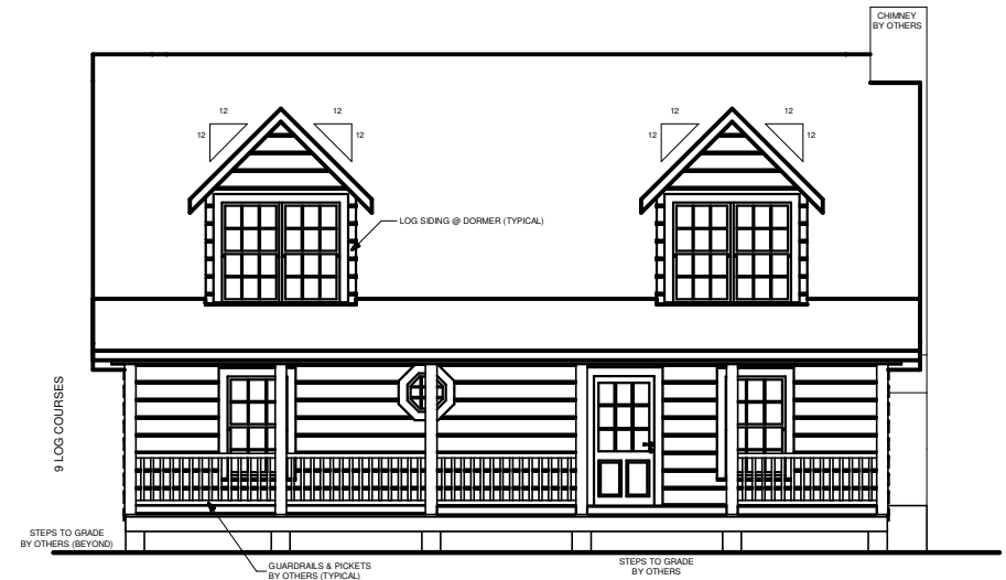
FRONT ELEVATION 1/4" = 1'-0"
