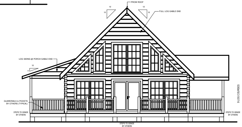
FRONT ELEVATION
