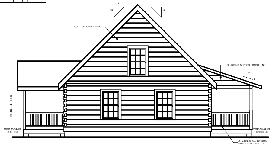
REAR ELEVATION
