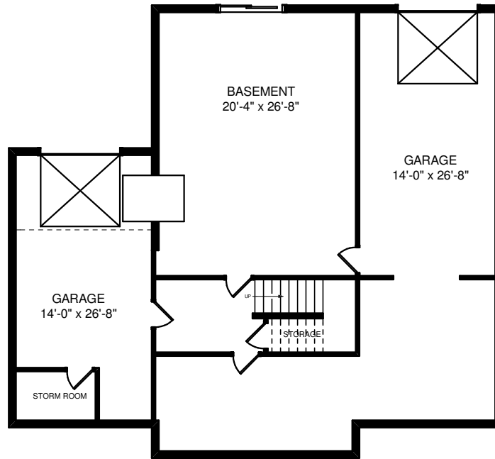
BASEMENT PLAN
