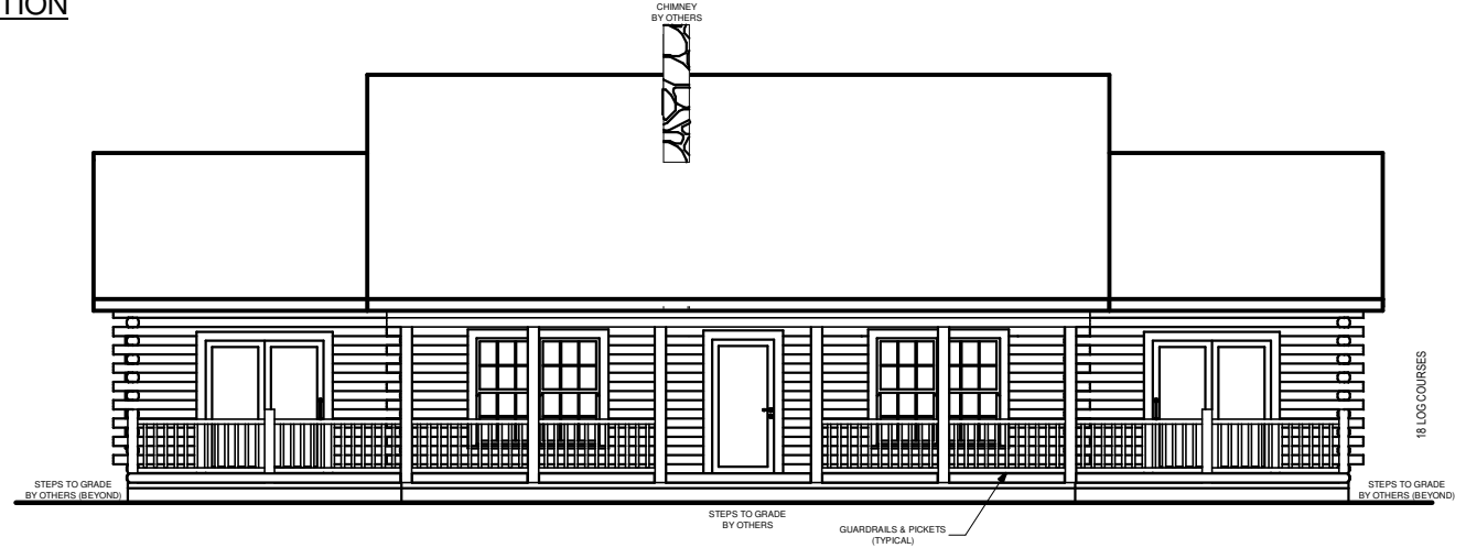
FRONT ELEVATION
