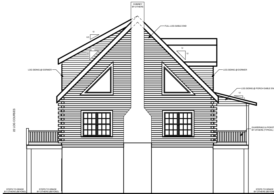
LEFT ELEVATION
