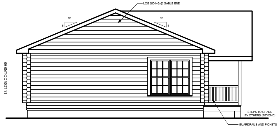
LEFT ELEVATION
