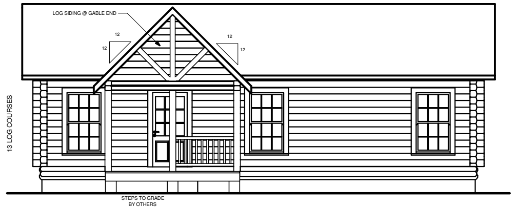
FRONT ELEVATION
