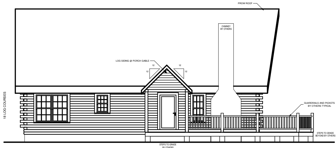
LEFT ELEVATION
