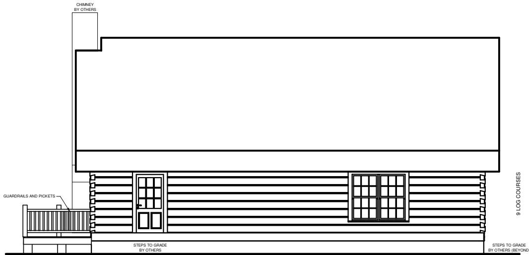
LEFT ELEVATION
