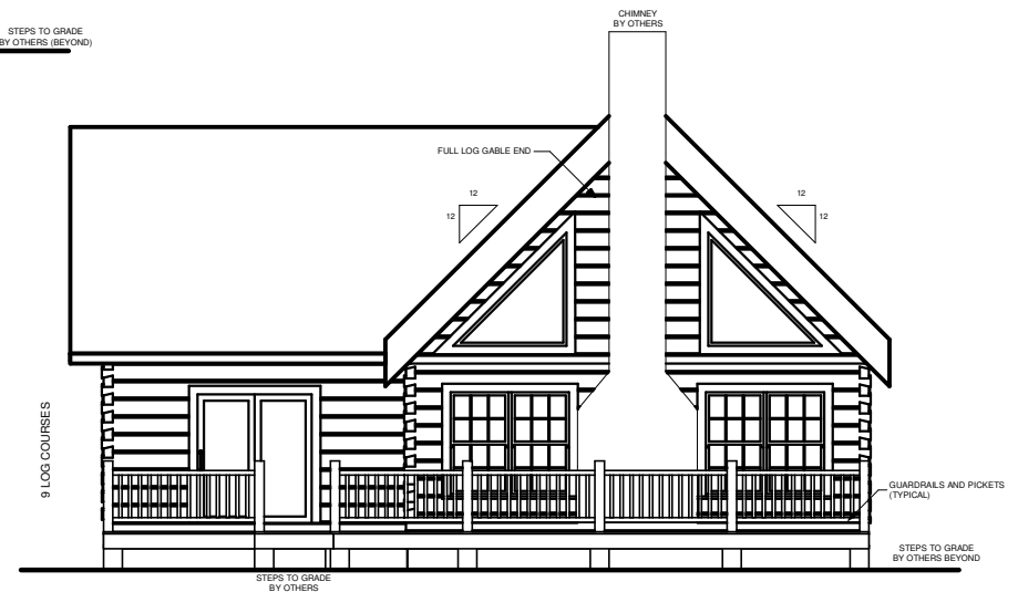
REAR ELEVATION
