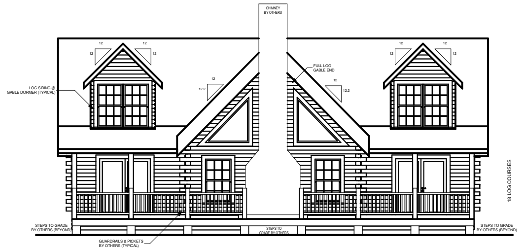
REAR ELEVATION
