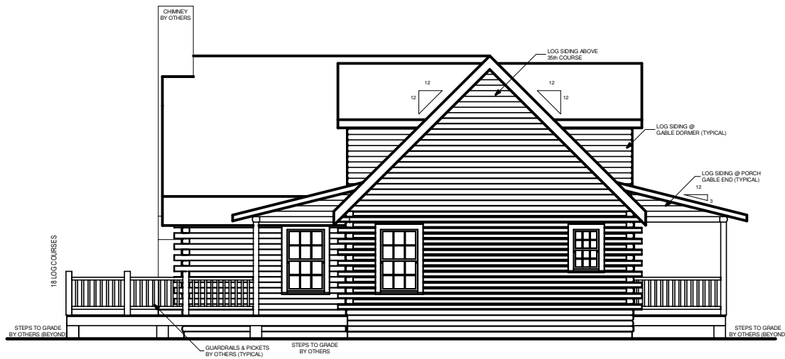
LEFT ELEVATION
