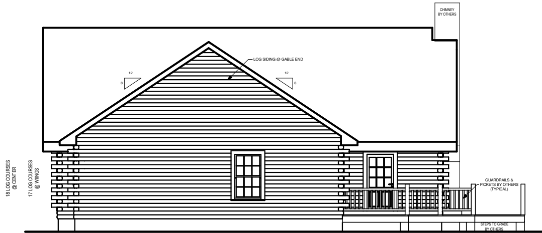
LEFT ELEVATION
