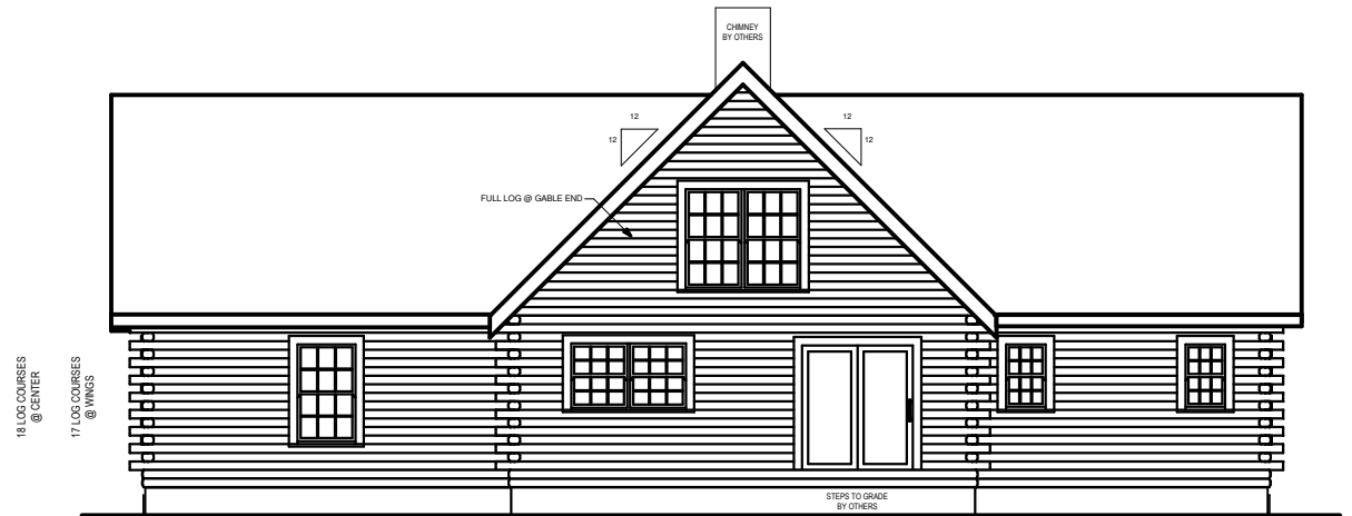
REAR ELEVATION
