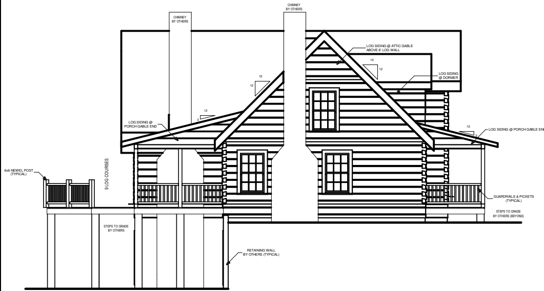
LEFT ELEVATION
