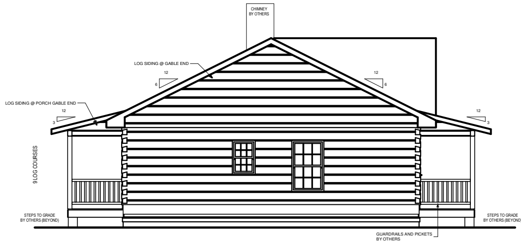
LEFT ELEVATION
