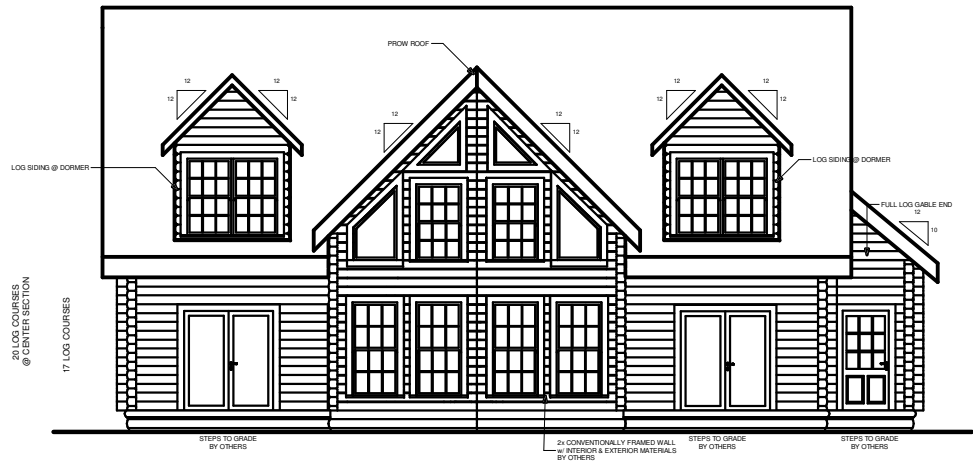
REAR ELEVATION
