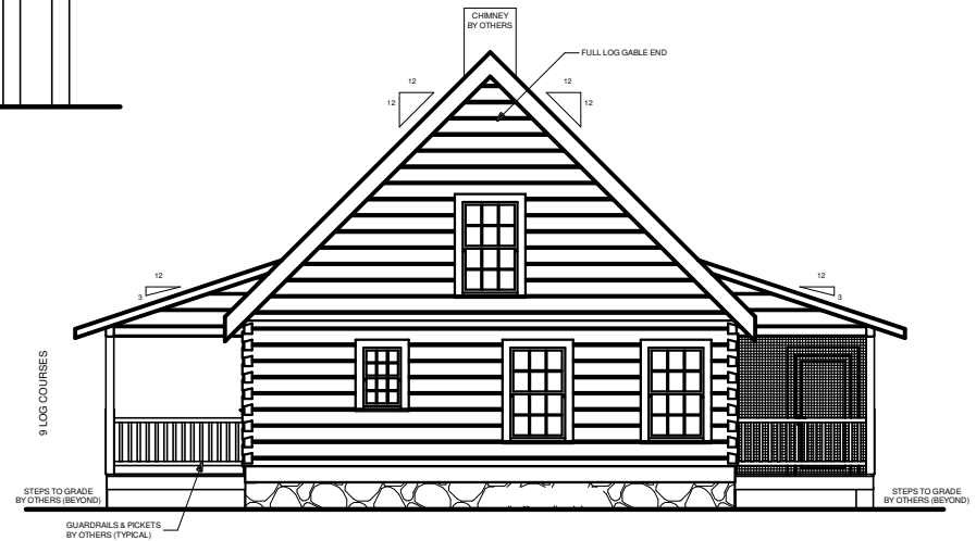
REAR ELEVATION
