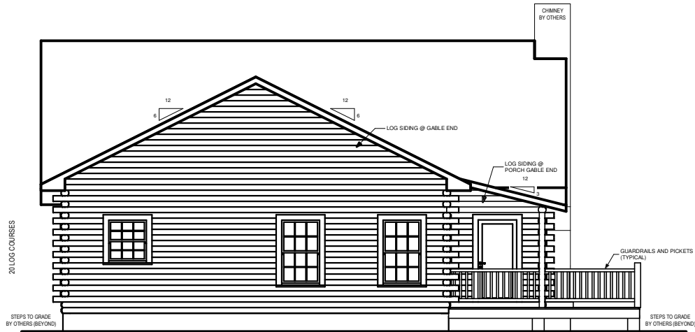
LEFT ELEVATION
