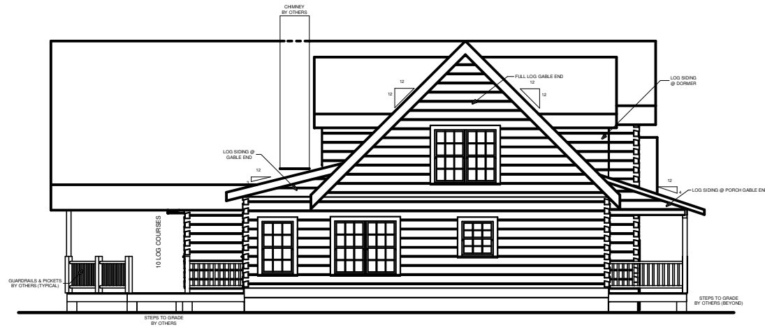
LEFT ELEVATION
