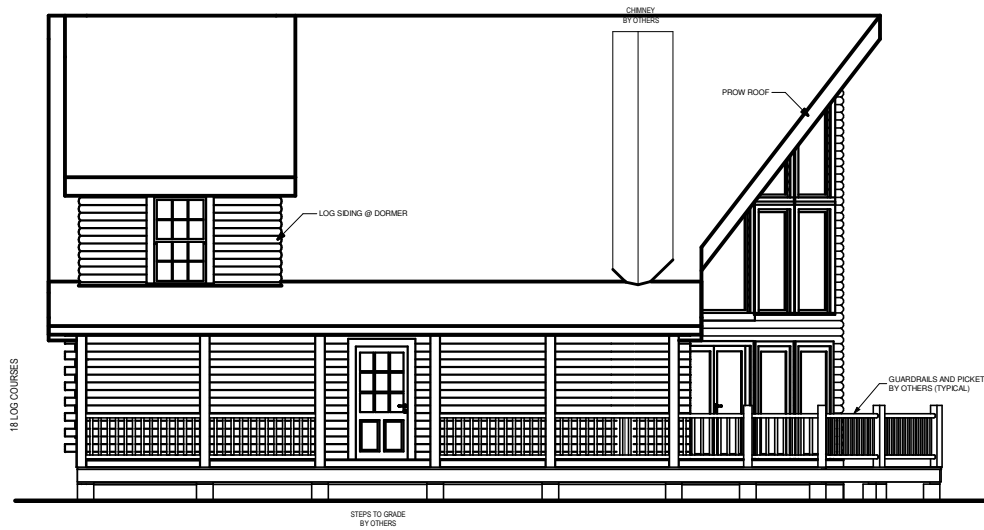
LEFT ELEVATION
