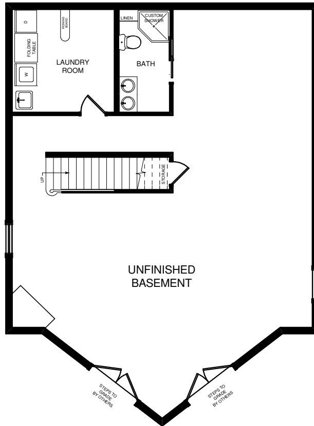
BASEMENT PLAN
