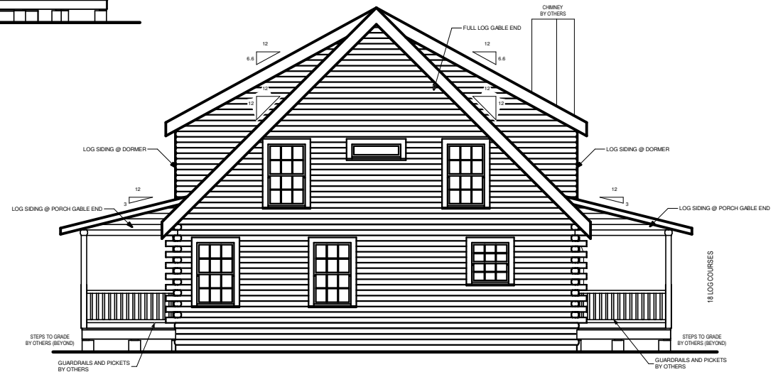
REAR ELEVATION
