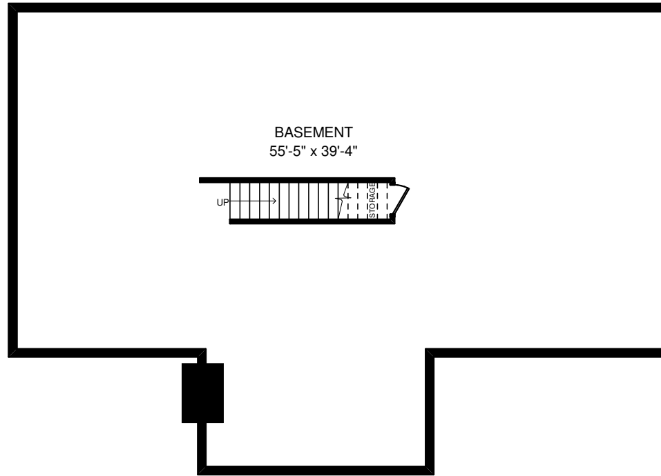
BASEMENT PLAN
