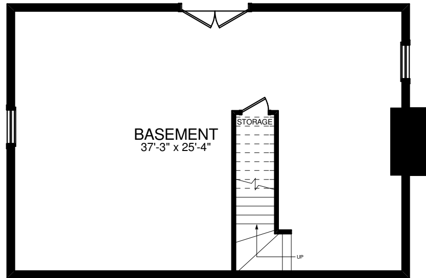
BASEMENT PLAN
