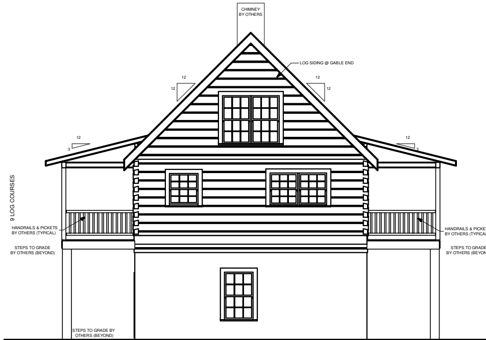
LEFT ELEVATION
